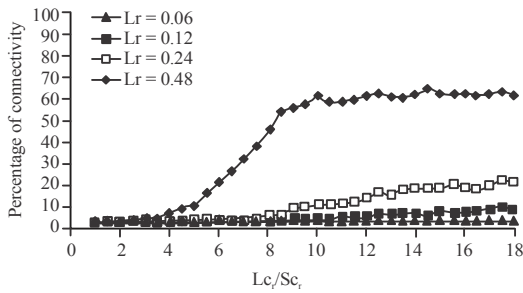
Fig. 5: Measurements of sensor nodes connectivity in the network at N_d = 80 , Lc_r = 3-50 m, Sc_r = 3 m (calculations of connectivity average over 30 runs)
