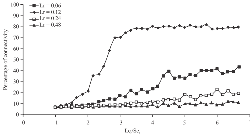
Fig. 7: Measurements of sensor nodes connectivity in the network at N_d = 80 , Lc_r = 7-50 m, Sc_r = 7 m (calculations of connectivity average over 30 runs)
