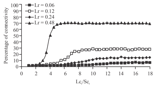
Fig. 6: Measurements of sensor nodes connectivity in the network at N_d = 400 , Lc_r = 3-50 m, Sc_r = 3 m (calculations of connectivity average over 30 runs)
