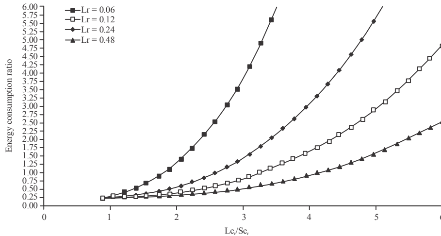
Fig. 4: Ratio of consumed energy by nodes at \lambda = 3 , S_r = 8 m, S_c = 7 m, L_c = 7-50 m
