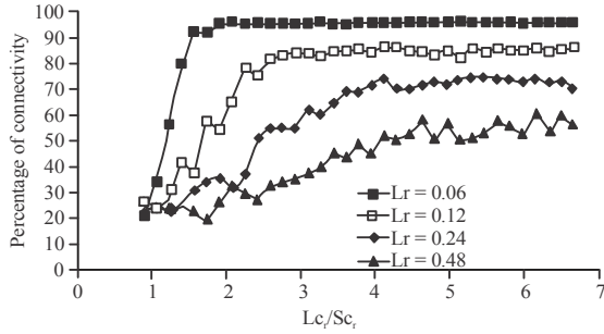
Fig. 8: Measurements of sensor nodes connectivity in the network at N_d = 240 , L_c = 7-50 m, S_c = 8 m (calculations of connectivity average over 30 runs)
