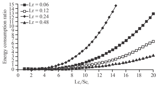
Fig. 3: Ratio of consumed energy by sensor nodes at \lambda = 3 , S_c = 8 m, S_r = 3 m, L_c = 3-50 m
