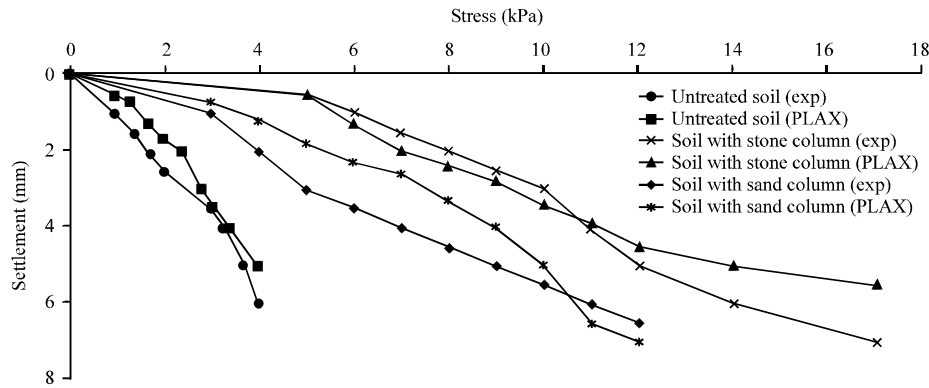
Fig. 12: Comparison of stress-settlement relations for clay treated with group of 8 columns ( s = 2.5 d )
