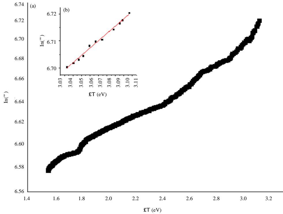
Fig. 7a, b): Natural logarithm of a vs. the incident photon energy for 9 wt.% composite
