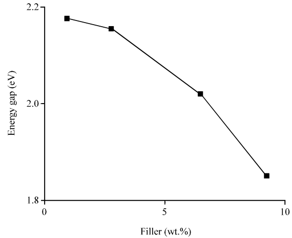
Fig. 3: Variation of the optical energy gap with oil ZnO concentrat
