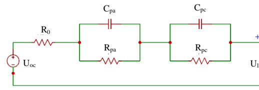
Fig. 3: Thevenin model (second order)
