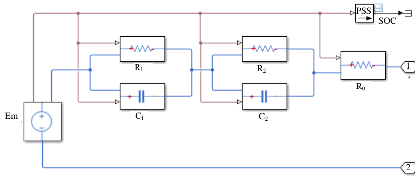
Fig. 4: Second order Thevenin Model with variable components
