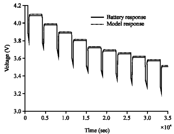
Fig. 9: Measured vs. estimated response after parameters identification
