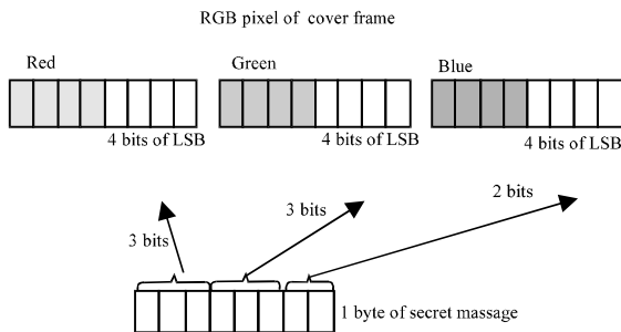
Fig. 3: Proposed LSB embedding technique, shows secret data embedded in 4 bits of LSB in 3, 3, 2 order in corresponding RGB pixels of the carrier frame
