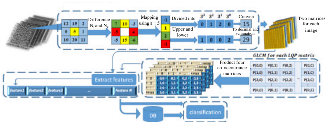
Fig. 8: Framework of LQP-CM
