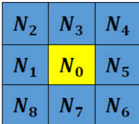
Fig. 2: The 8-neighbours
