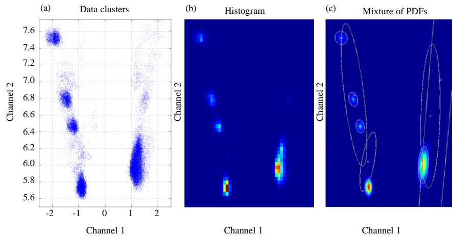
Fig. 5: a-c) Representation of data clusters (left diagram) by histogram (middle diagram) and by mixture of probability density functions (pdfs)
