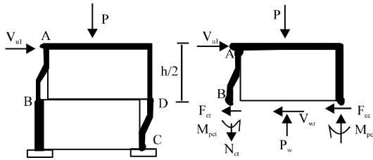
Fig. 18: Mechanism 1
