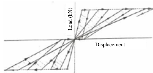
Fig. 11: Hysteretic model of clay blocks; Hollow clay blocks
