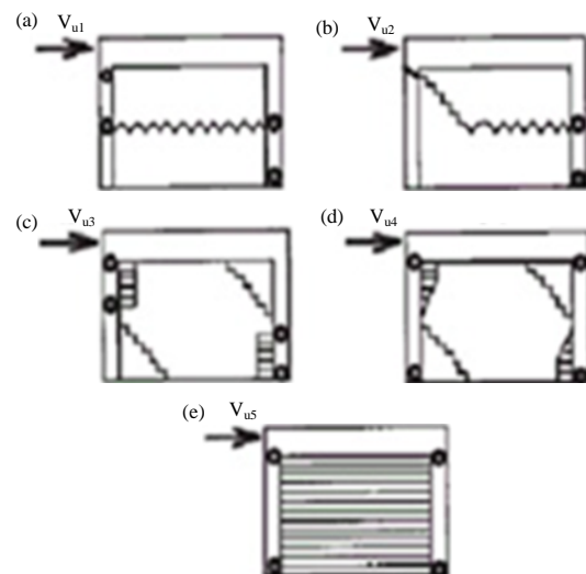
Fig. 17a-e: Most probable failure modes (Mehrabi and Shing, 1994)
