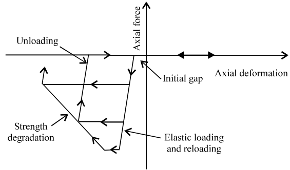
Fig. 14: Hysteretic model presented by Doudoumis and Mitsopoulou (1986)
