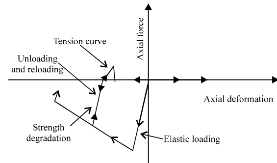
Fig. 15: Hysteretic model proposed by Andreaus et al. (1985)
