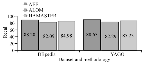
Fig. 4: Performance evaluation of the methodologies on recall against the different datasets
