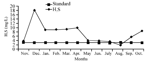
Fig. 8: Concentration of effluent H 2 S compared with the standard Iraqi specification
