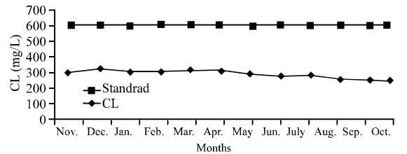
Fig. 10: Concentration of effluent CL compared with the standard Iraqi specification
