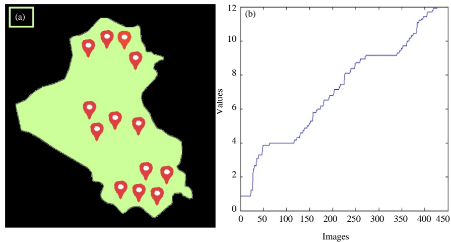
Fig. 9: K-function on sample points of Iraqi map: a) Input image map and b) Output graph
