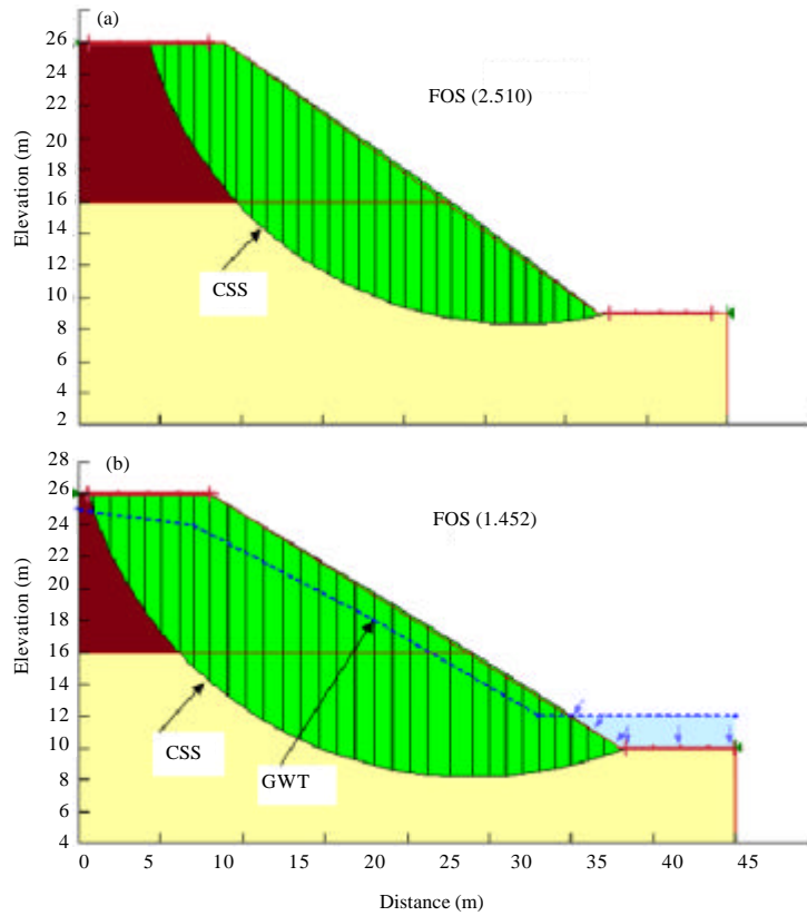
Fig. 12: Non-optimised: a) Dry and b) Wet slopes for Oko 1 and 2 (Anambra State)
