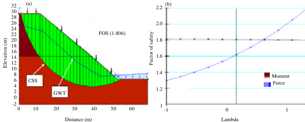
Fig. 17: a) Optimised slope with point load of 40 kPa and b) Plot of FOS versus lambda, (optimised) with external loads of 40 kPa
