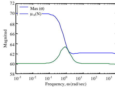
Fig. 17: Robust performance
