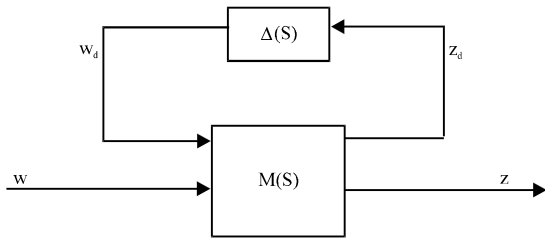
Fig. 5: M-Δ structure
