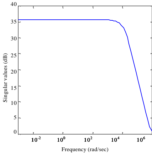
Fig. 15: Nominal stability
