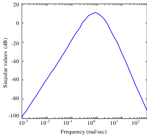
Fig. 16: Robust stability
