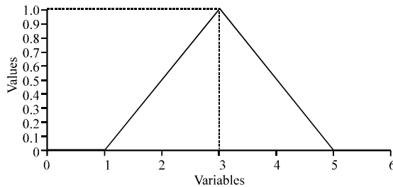
Fig. 2: Numerical example ( \tilde{A}=(1, 3, 5) )
