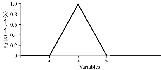
Fig. 1: Triangular fuzzy number ( \tilde{A}=(a_1, a_2, a_3) )
