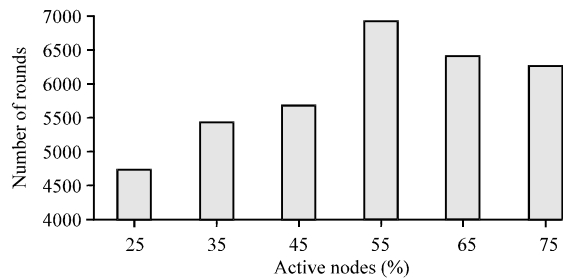
Fig. 4: Life time of DPMC
