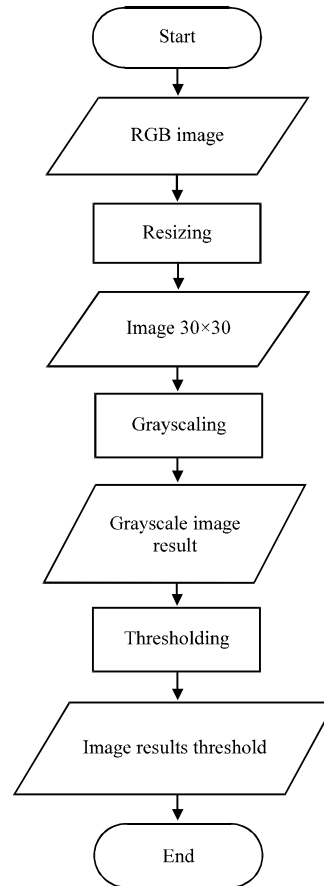
Fig. 2: Pre-processing
