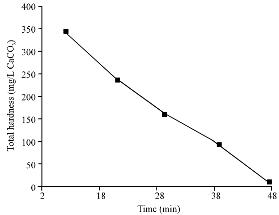
Fig. 2: Total hardness value (mg/L CaCO 3 ) after adding the lime to the hard water sample
