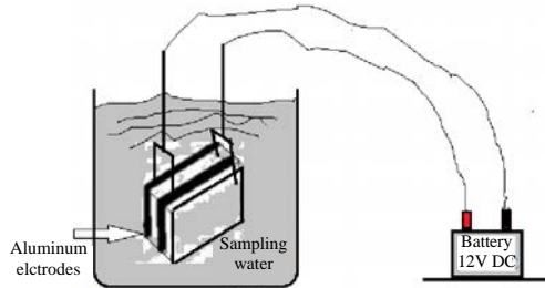
Fig. 1: Electrolytic cell block diagram
