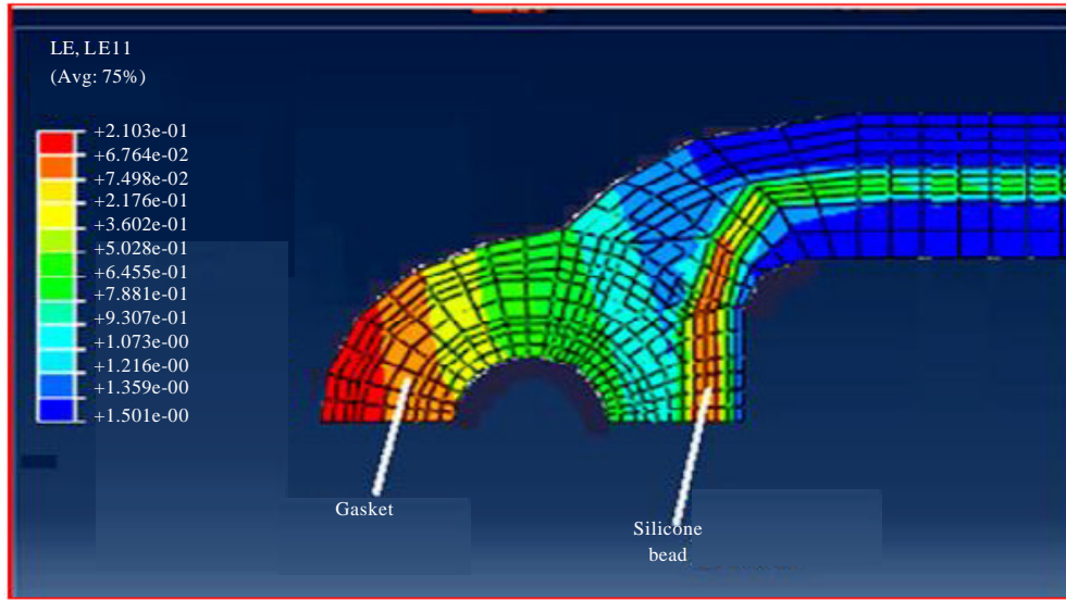
Fig. 14: Contour of strain along the periphery of gasket
