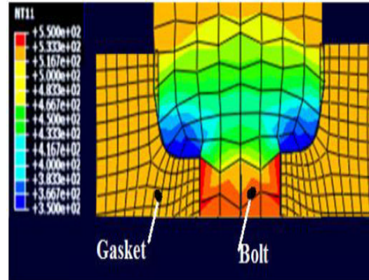
Fig. 13: Magnified contour of nodal temperature near combustion chamber
