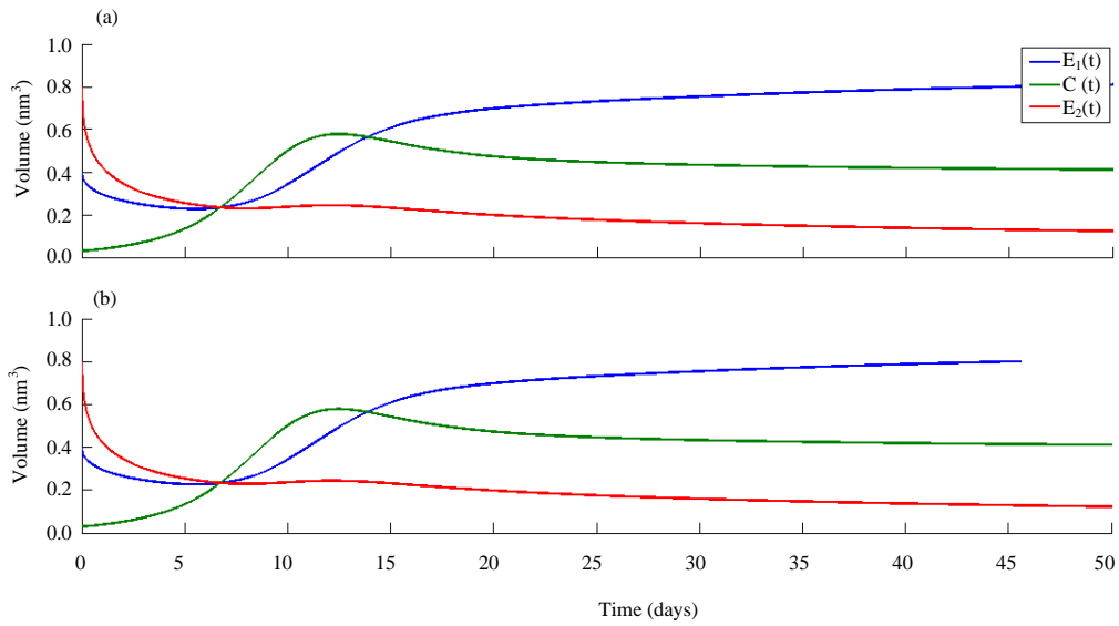
Fig. 3: Numerical results for Eq. 19 and 20 when \alpha = 0.5 , d_1 = 0.3, 0.7 , d_2 = 0.7 , k_1 = 0.3 , k_2 = 0.7 : a) Implicit Euler method and b) Predictor-corrector method
