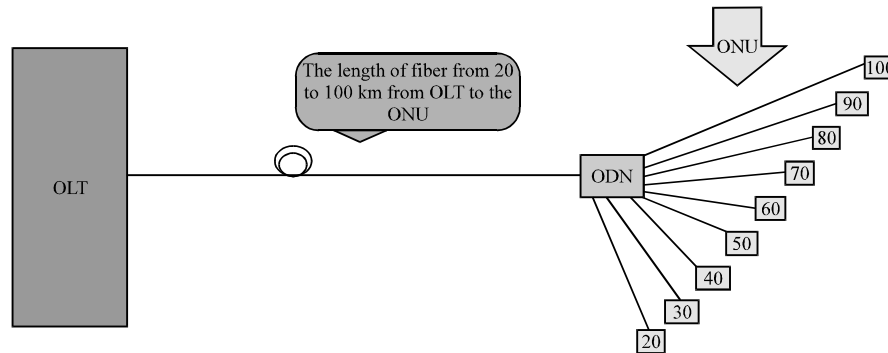
Fig. 8: GPON-FTTx representing a distribute ONU among available distance
