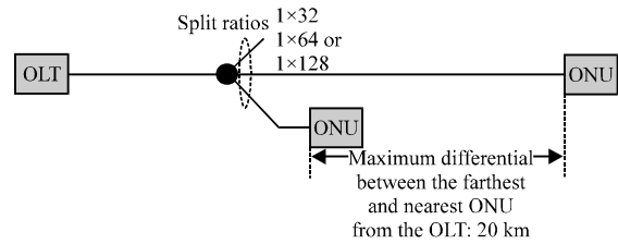
Fig. 4: Gigabit Passive Optical Network (GPON) shows the three main section in any PON the OLT which represent the source, ODN which represent the splitter with the fiber (range from 20-90) and ONU which represent the destination (Bakarman et al. , 2010)
