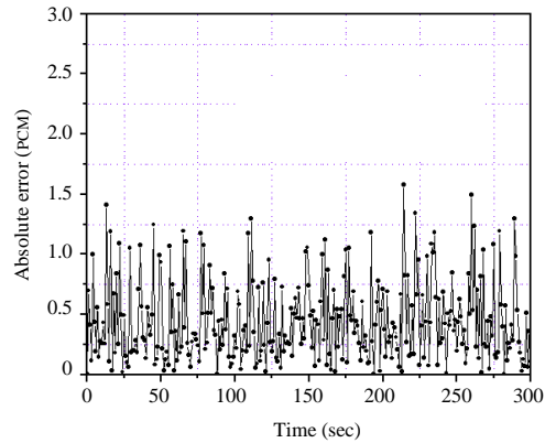
Fig. 6: Variation on the absolute error over time for a neutron population density of the form P(t) = a+bt^4 with a = 1 and b = (0.0127)^5/9 with a time step T = 0.01 s of using the FIR filter and the low-pass filter ( \sigma = 0.01 , \tau = 0.5 , sample number, mean absolute error = 0.36 PCM)
