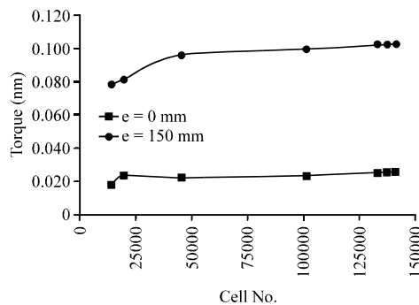
Fig. 5: Variation of static torque with respect to number of cells from the grid independence test at rotor angle of 0° (3-blade rotor, H = 500 mm, d = 160 mm)
