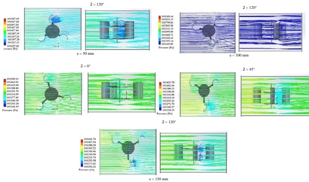
Fig. 10: Pressure distribution for 3-bladed rotor versus rotor positions
