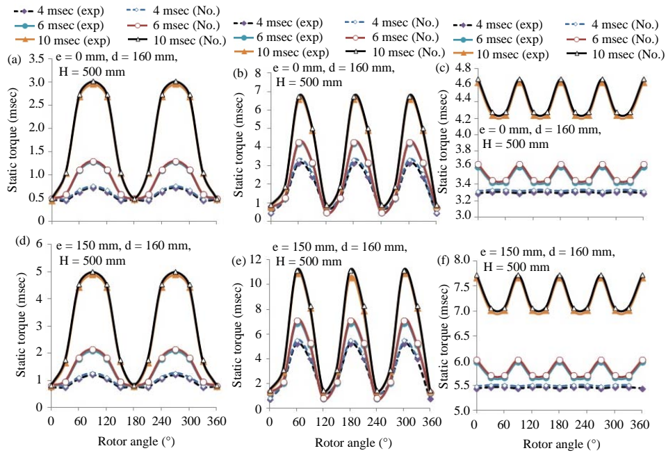
Fig. 7: Static torque vs. rotor positions: a, d) 2-blade; b, e) 3-blade and c, e) 4-blade
