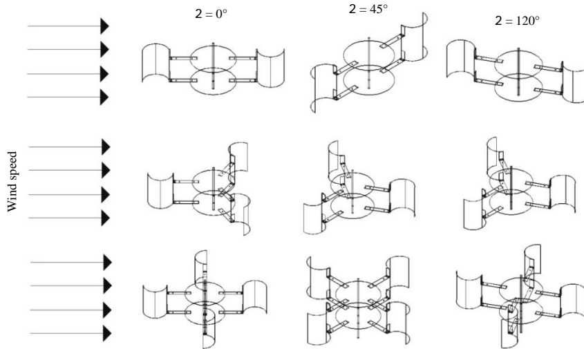
Fig. 8: Rotor positions
