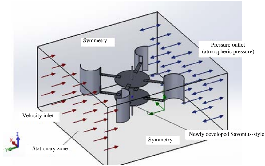
Fig. 3: Computational domains with boundary conditions
