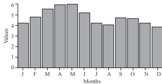
Fig. 6: Solar irradiation and time; monthly average daily irradiation, horiz, surface
