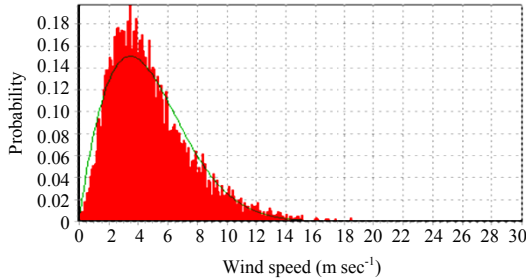
Fig. 7: Wind speed and time (Case 2. Location-Rajasthan)
