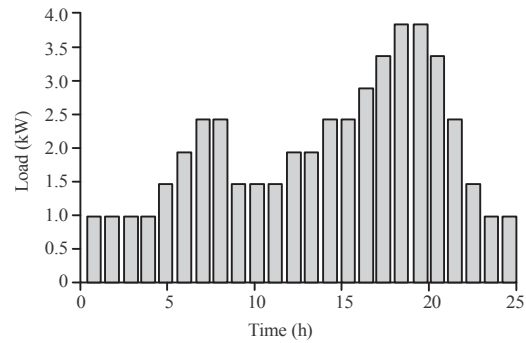
Fig. 4: Load profile
