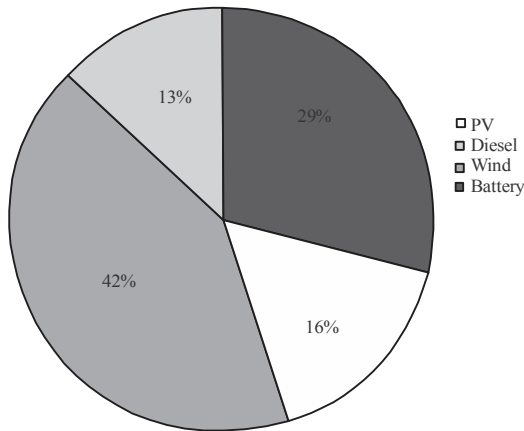
Fig. 13: Power output contribution of power output PV, wind, battery, diesel for Tamil Nadu location (Location 3: Tamil Nadu)
