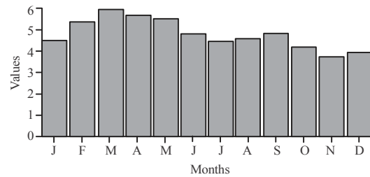
Fig. 10: Solar irradiation and time; monthly average daily irradiation, horiz, surface
