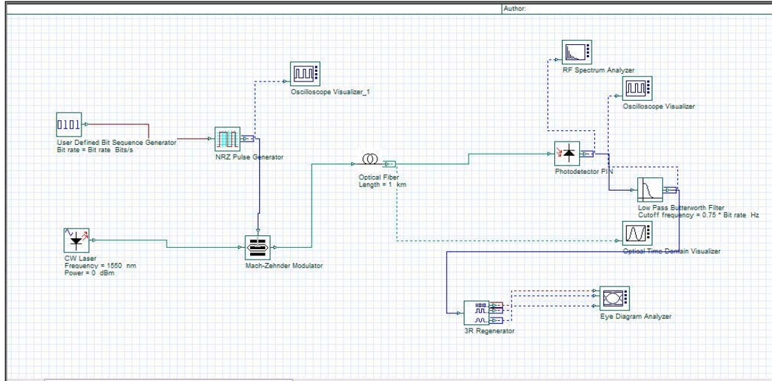
Fig. 2: The simulation system
