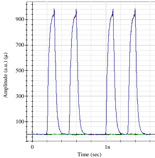
Fig. 4: The received signal at 1 km optical fiber
