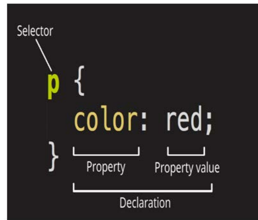
Fig. 3: Example of CSS syntax
