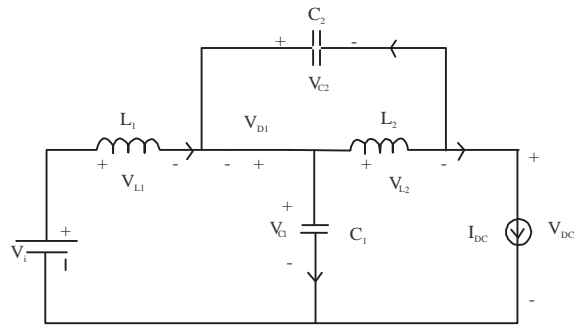
Fig. 3: Equivalent circuit for non-shoot through state
