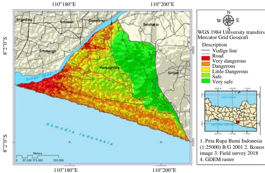
Fig. 3: Tsunami Hazard of Parangtritis village, Kretek, Bantul, D.I. Yogyakarta
