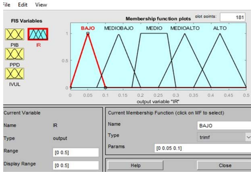
Fig. 2: Parameters of population growth rate
