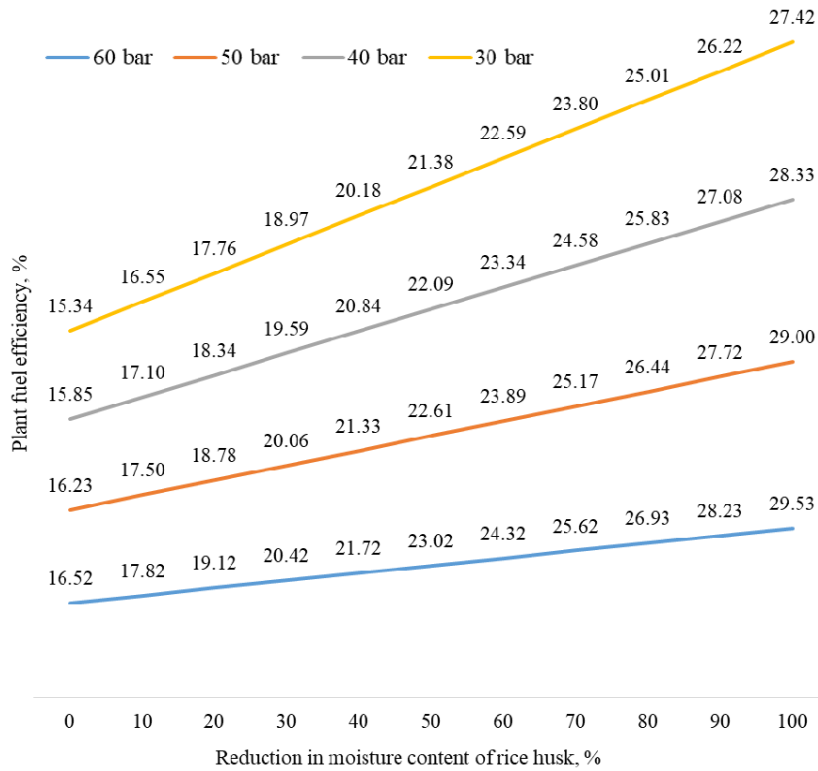
Fig. 9: Plant fuel efficiency vs. moisture reduction [4]
