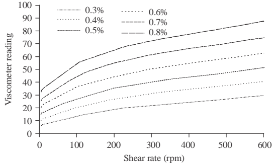
Fig. 1: Rheology of biopolymer solutions of xanthan gum with a concentration of 0.3-0.8%
