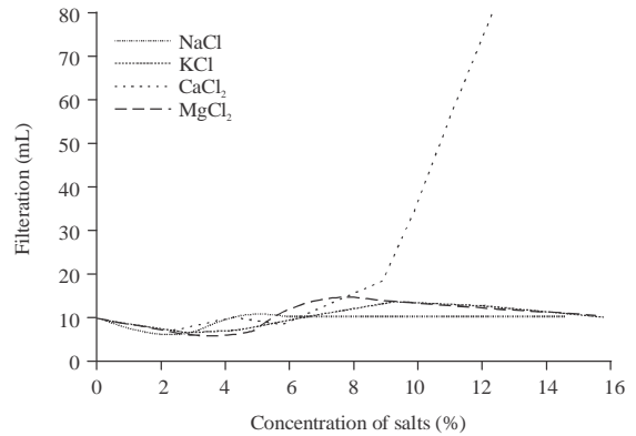
Fig. 4: The dependence of filtration on the salt concentration of the polymer solution of 0.5% xanthan gum
