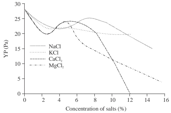
Fig. 3: The dependence of Yield Point (YP) on the salt concentration of the polymer solution of 0.5% xanthan gum
