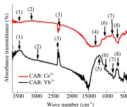
Fig. 2: FTIR spectra of CAB:Yb 3+ and CAB:Ce 3+ glasses. The peaks were identified according to Table 1
