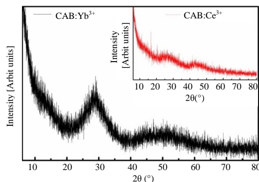
Fig. 1: XRD pattern of glass CAB: Yb 3+
