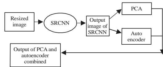
Fig. 1: Framework
