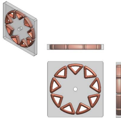
Fig. 3: Stator design of double side axial flux permanent magnet generator
