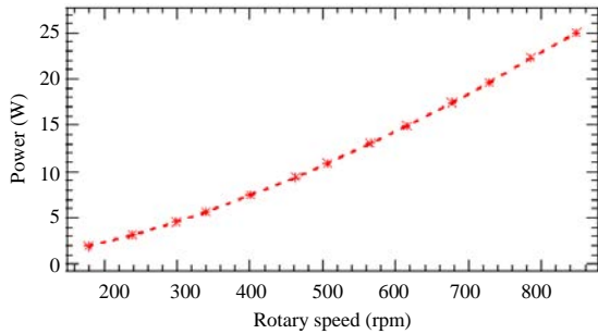
Fig. 9: Correlation between output power and rotational speed
