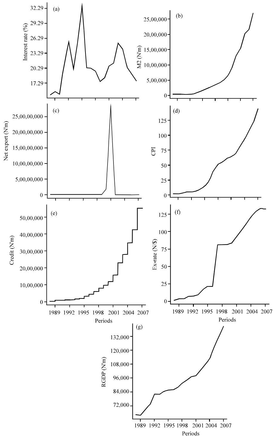
Fig. 1: Trend analysis
