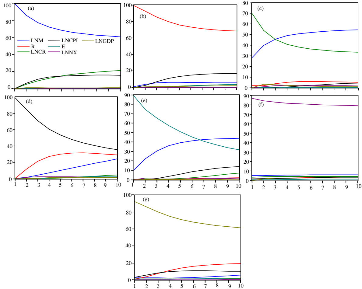
Fig. 3: Variance decomposition; a) LNM, b) R, c) LNCR, d) LNCPi, e) E, f) LNNX and g) LNGDP (1991 Act period)
