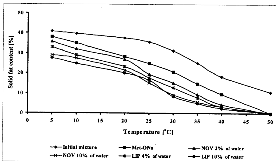
Fig. 1: The solid fat content (SFC) versus temperature for the initial mixture consisted of 50% soybean oil and 50% stearin and for TAGs isolated from fats after interesterifications catalyzed by sodium metoxide (Met-ONa), Novozyme 435 (NOV) and Lipozyme IM (LIP).
