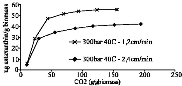
Fig. 3 Effect of the flow rate (superficial velocity) of supercritical CO 2 in SFE of astaxanthin from the yeast Phaffia rodozyma
