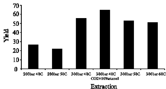
Fig. 7: Astaxanthin yield from the yeast Phaffia rodozyma by Supercritical CO 2 Extraction
