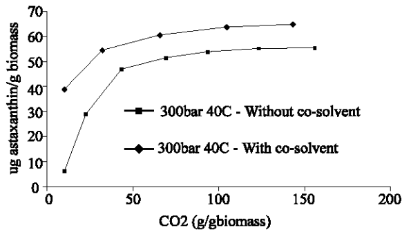
Fig. 2: Effect of the co-solvent ethanol (10%) on Supercritical CO 2 Extraction of astaxanthin from the yeast Phaffia rodozyma
