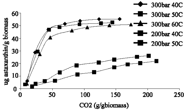
Fig. 1: Effect of pressure and temperature on Supercritical CO 2 Extraction of astaxanthin from the yeast Phaffia rodozyma
