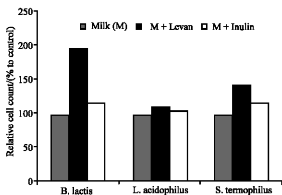
Fig. 2: Relative changes in cell count for individual constituents of ABT-5 on selective media during 12 h cultivation in milk supplemented by fructans. Cell count values in controls: 5.55 \pm 0.56 \times 10^6 ( B. lactis ); 6.30 \pm 0.65 \times 10^7 ( L. acidophilus ); 1.31 \pm 0.12 \times 10^9 ( S. thermophilus )
