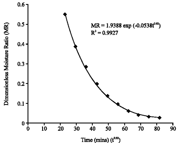
Fig. 2: Model of drying of cassava particulate at 50^\circ\text{C}
