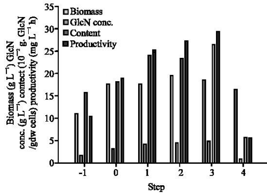
Fig. 4: Plots of GlcN concentration, biomass, GlcN content, productivity of Aspergillus sp. BCRC 31742 for producing GlcN as the effect of various WF sugar and peptone concentrations according to steepest ascent method
