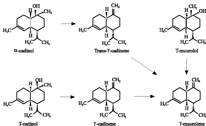
Fig. 1: Biotransformations of sesquiterpene alcohols to \gamma -muurolene
