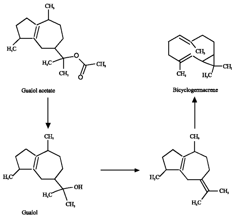
Fig. 2: Biotransformations of guaiol acetate to bicylogermacrene
