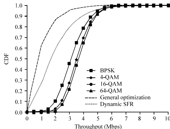
Fig. 2: Performance in cell-edge user
