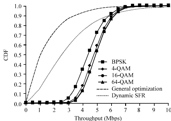
Fig. 3: Performance in cell-center user
