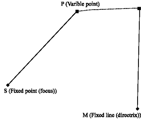
Fig. 1: Points representation
