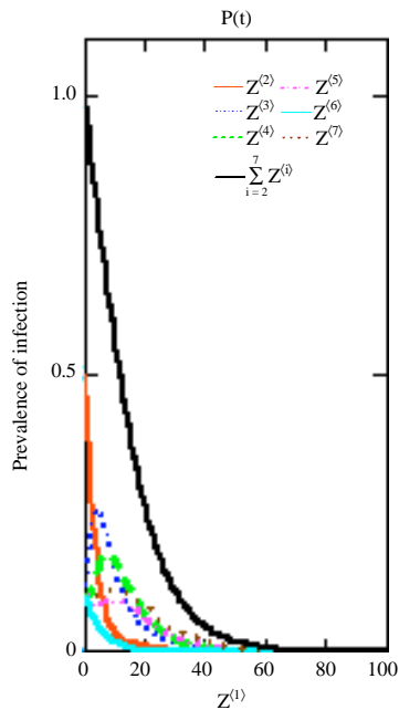
Fig. 3: Graphical simulations of s_p, l_i, u_i, w_i, x_i, y_i from model (Eq. 16-21) against time with Z^{(i)} the sum of proportions of various group populations, only IPT and bi-therapy were used. Parameter values are in variants (1 and 2) in Table 2
