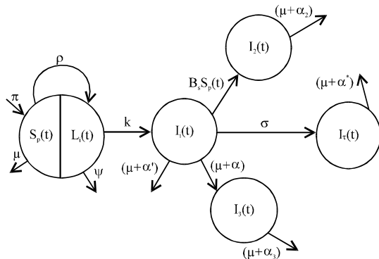
Fig. 1: A differential flow-chart for TB Bi-Therapy Treatment Model
