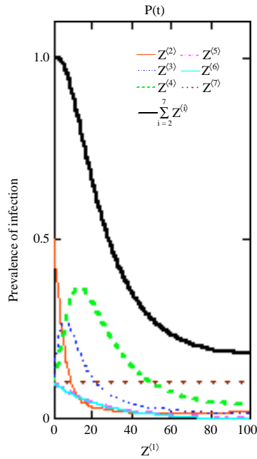
Fig. 2: Graphical simulations of s_p, l_i, u_i, w_i, x_i, y_i from model (Eq. 16-21) against time with Z^{(i)} the sum of proportions of various group populations, nobody used preventive measure. Parameter values are in variants (1 and 2) in Table 2
