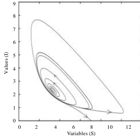
Fig. 3: An unstable periodic solution exist where A = 8 , d = 0.1 , \nu = 1 , \gamma = 1 , r = 5.1
