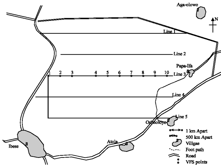
Fig. 2: Base Map of the study area (Ibeshe)
