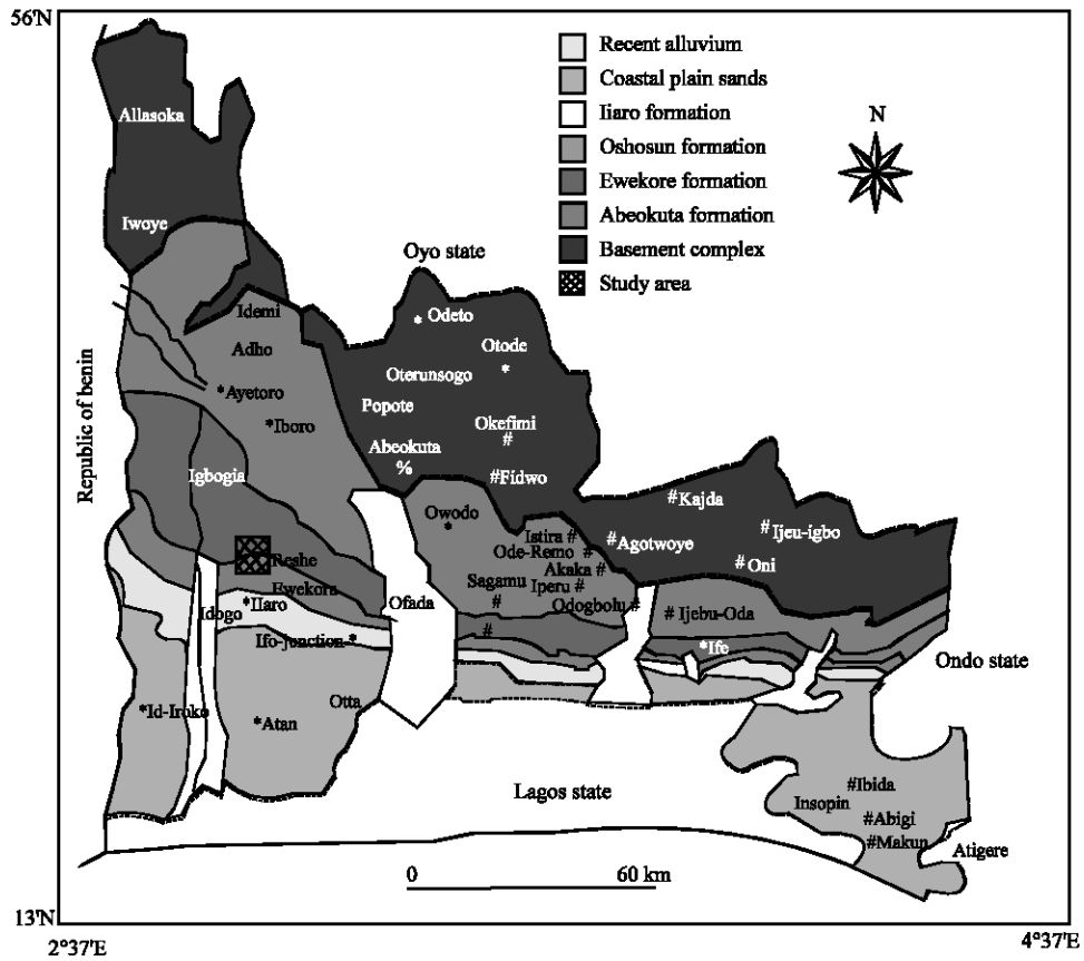
Fig. 1: Shows Geologic Map of Ogun State showing the major geologic formations around Ibeshe, the Study Area
