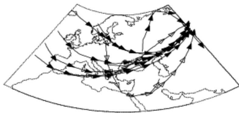
Fig. 7: The average of the main paths of 500 hPa Jetstreams
