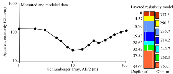
Fig. 2: Iterated field curve and the apparent resistivity model of VES 1
