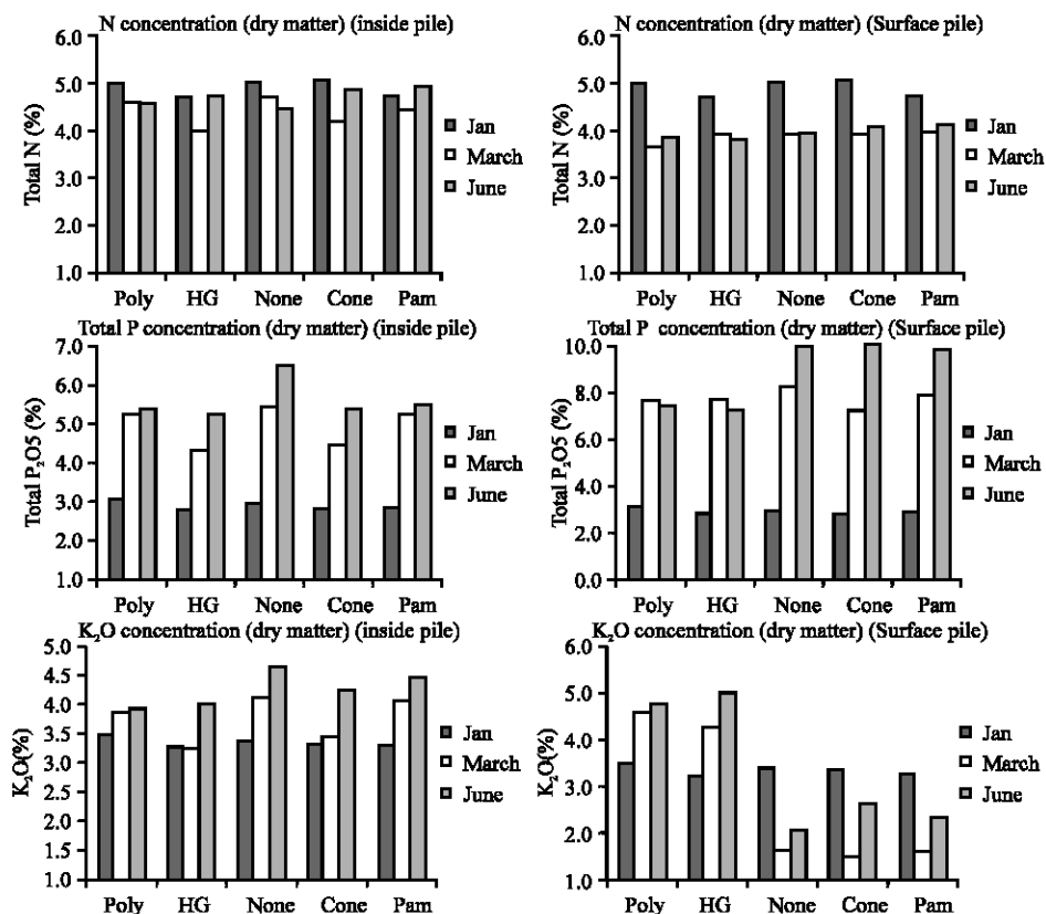
Fig 6: Nitrogen, P and K in dried litter from samples collected on the surface (6 in.) of the piles and from inside the piles (3 ft) as affected by storage treatment
