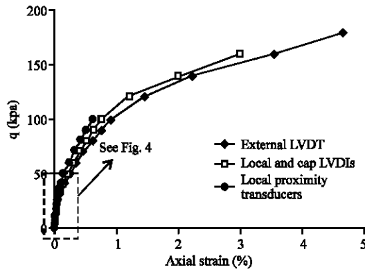
Fig. 2: Behaviour of the soil at small-intermediate strains level (0-5%)
