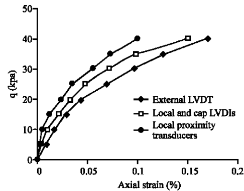
Fig. 4: Behaviour of the soil at small strains level (0-0.2%)
