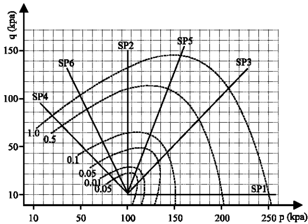
Fig. 5: Strain energy contours (Series 1)
