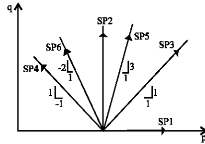
Fig. 3: Stress path orientations investigated
