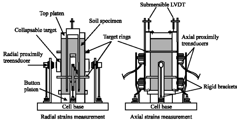
Fig. 1: Arrangement of the local strain measurement devices
