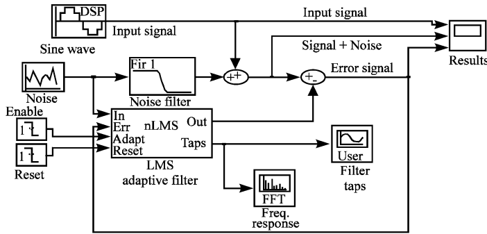
Fig. 1: Diagram showing the adaptive filter system
